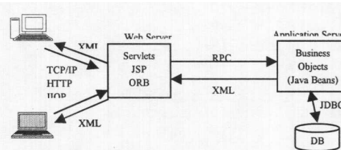
Figure 4: Sample 3-Tier Web Application Architecture
